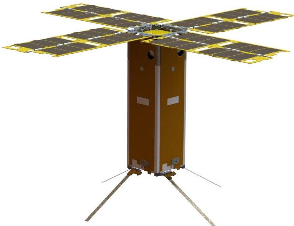
Example end hinge array using 90° hinges
