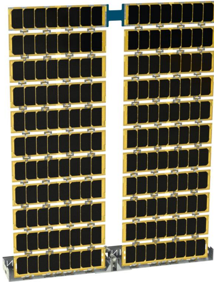
Deployable Clamshell Solar Array (DCSA) 11-Panel
